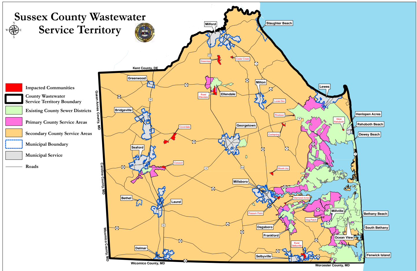
Figure 15: County Wastewater Service Territory
